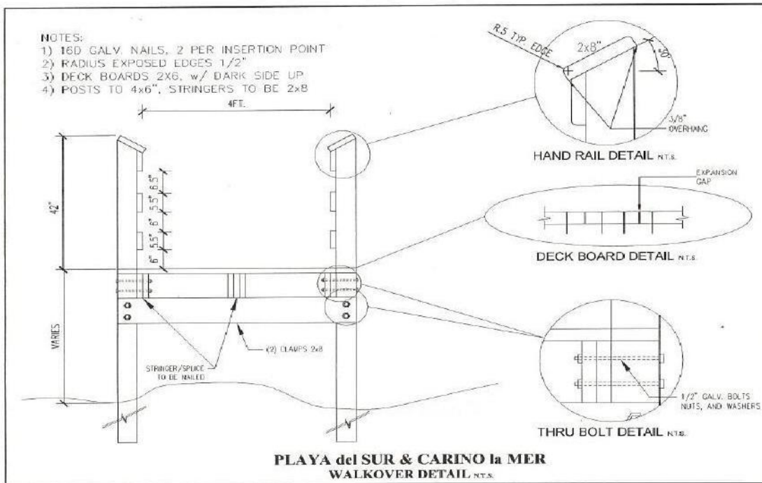
FIGURE 2 Walkover Details
